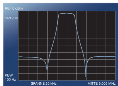
3-kHz-Roofing-Filter (9 MHz, SPANNE: 20 kHz)
