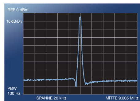
300-Hz-Roofing-Filter (9 MHz, SPANNE: 20 kHz)
